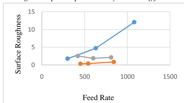
Fig 6: Graph: Surface Roughness v/s Feedrate
