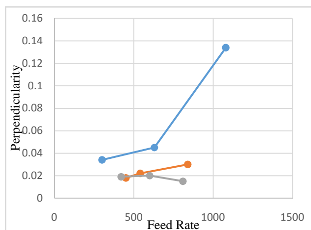
Fig 7: Graph: Perpendicularity v/s Feedrate
